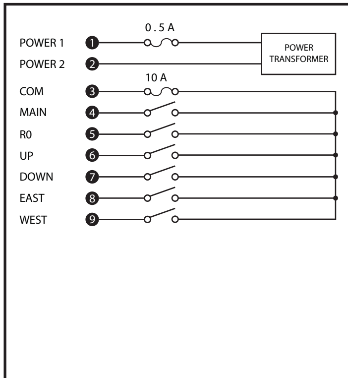
Q400 Wiring diagram
