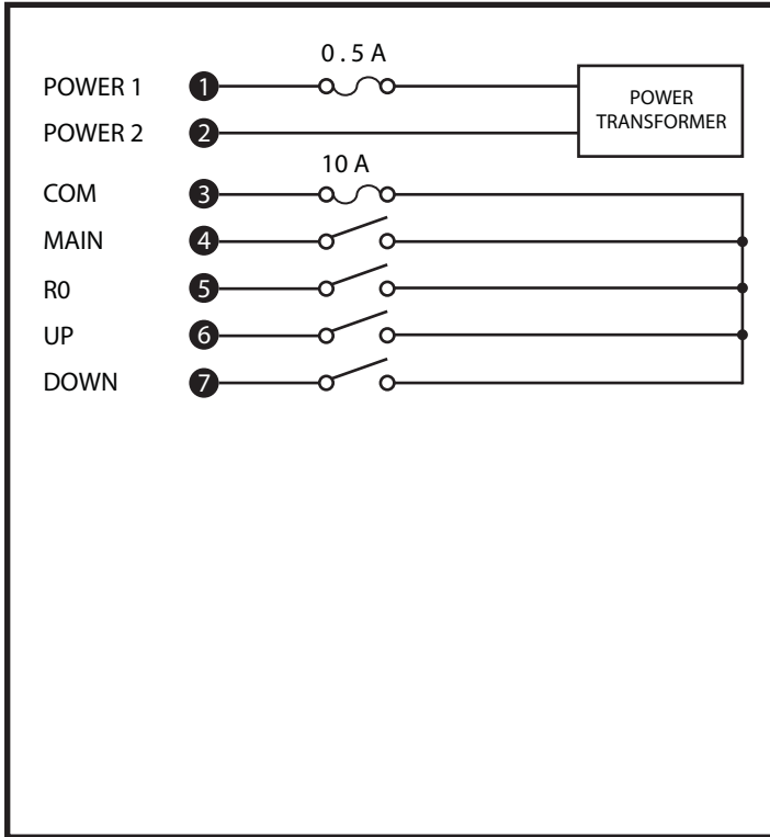
Q200 Wiring diagram
