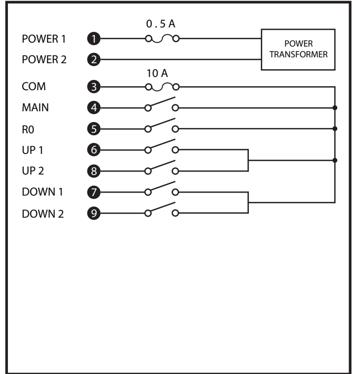
Q202 Wiring diagram
